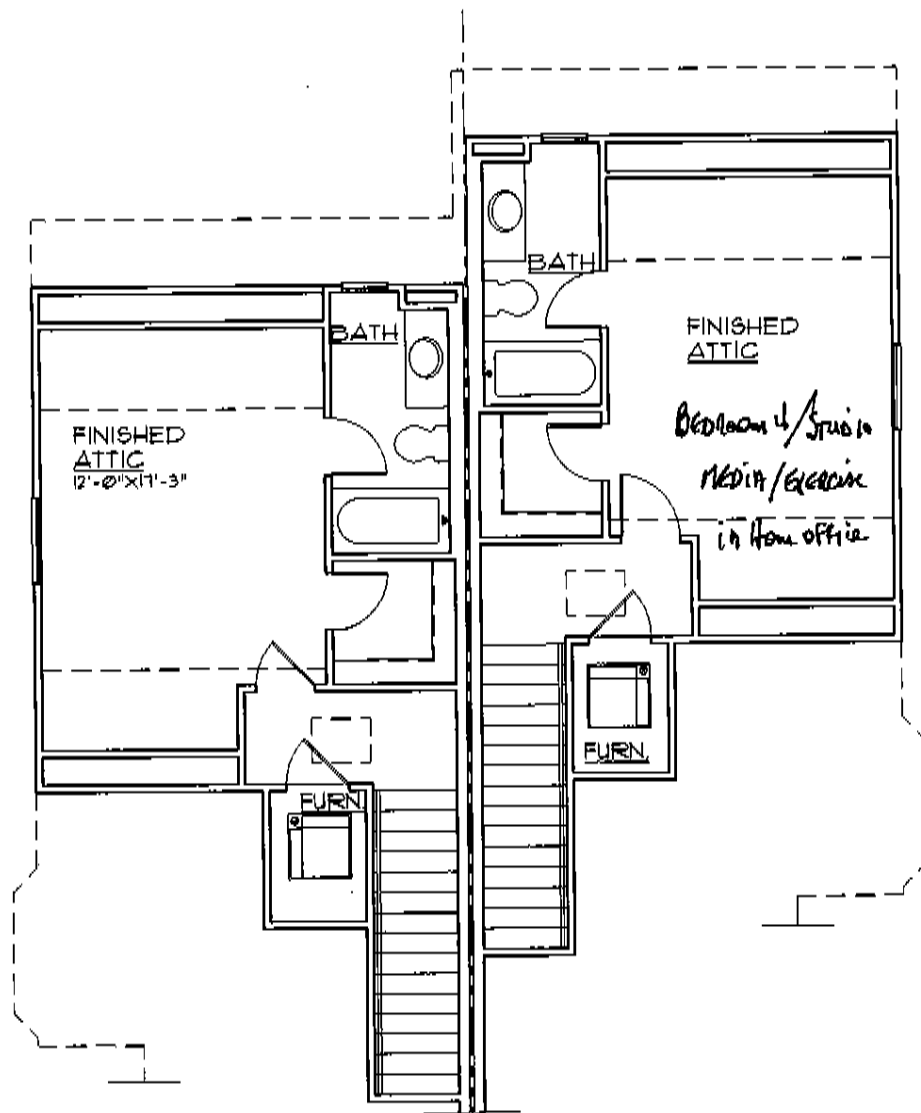
ATTIC LEVEL PLAN
